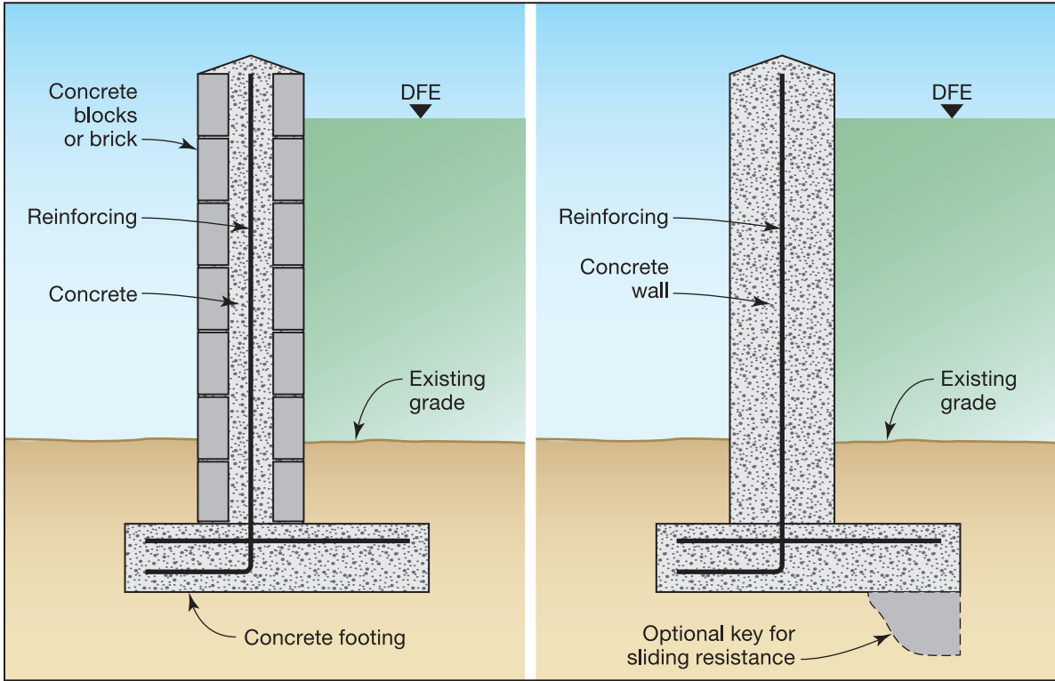
Figure 5F-6. Concrete cantilever floodwall reinforcement
