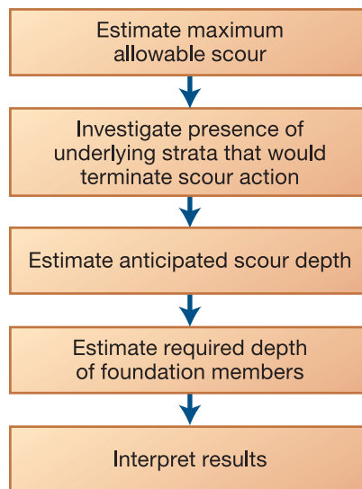
Figure 4-25. Process for estimating potential scour depth
