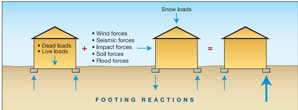
Figure 5-4. Foundation system loading
