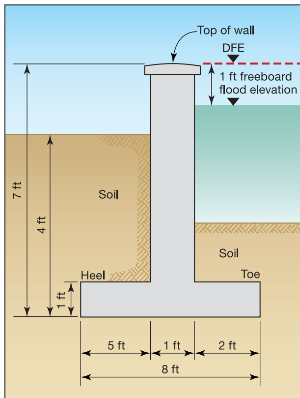
Figure 6-46. Floodwall dimensions for the Valley house floodwall
