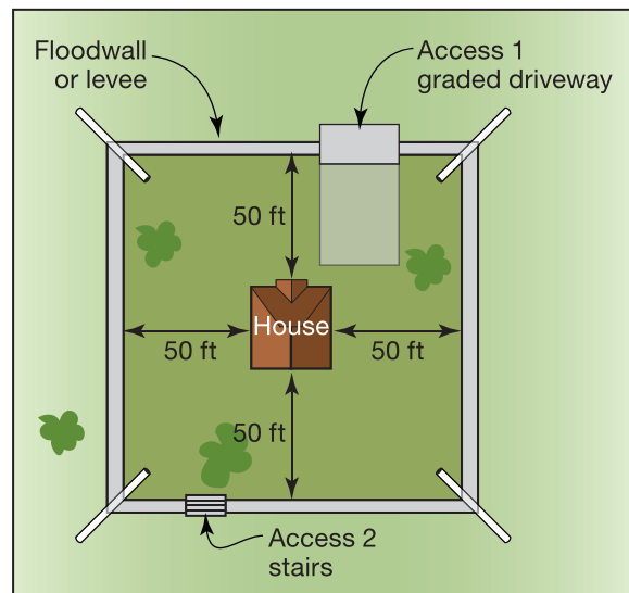
Figure 6-47. Plan drawing for Valley house floodwall or levee
