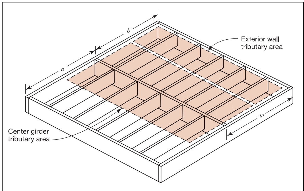
Figure 5-7. Wall/girder tributary area
