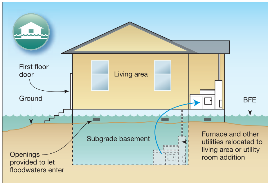
Figure 1-10. Wet floodproofed structure
