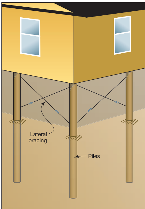
Figure 1-5. Elevation on piles
