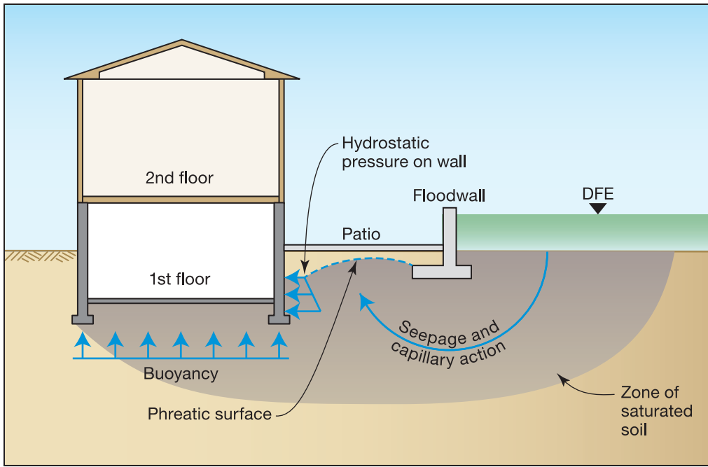
Figure 5F-9. Seepage underneath a floodwall
