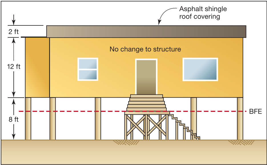
Figure 6-20. The Chester house, after mitigation
