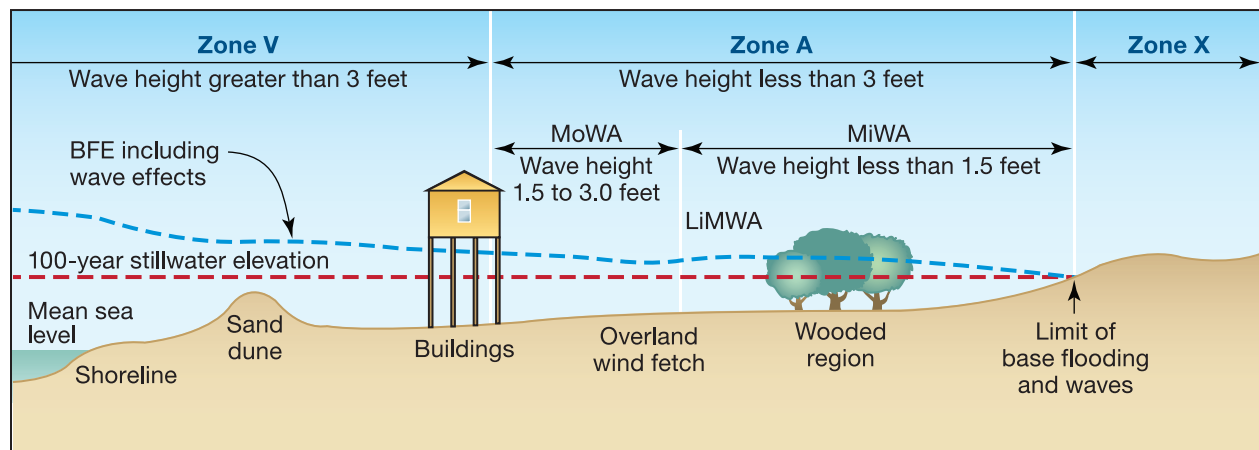
Figure 2-4. Wave height transect showing LimWA, MoWA, and MiWA
