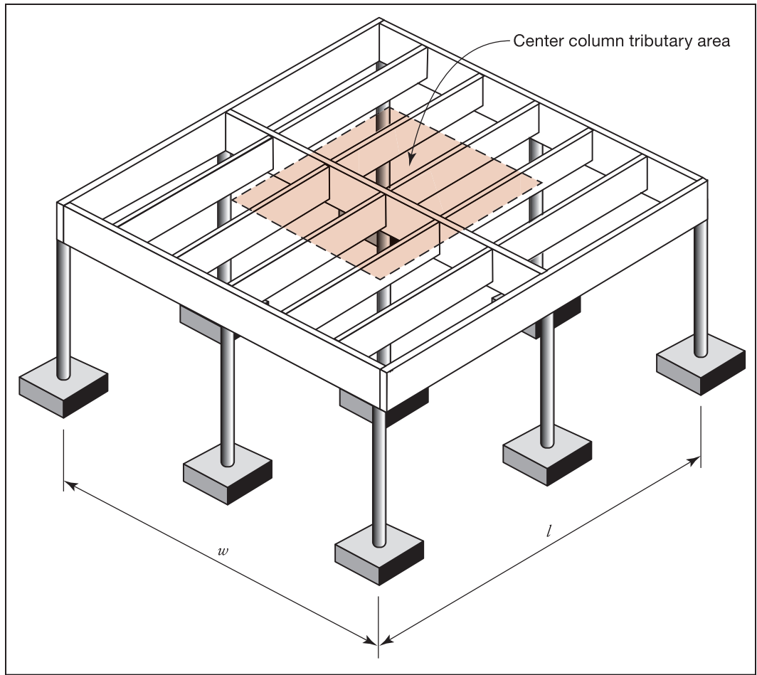
Figure 5-6. Column tributary area
