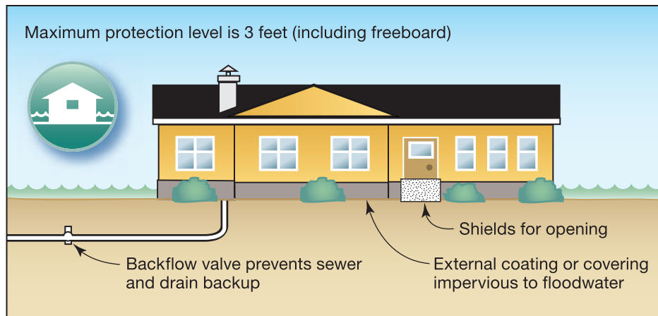
Figure 1-9. Dry floodproofed structure
