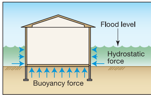
Figure 3-7. Hydrostatic and buoyancy forces
