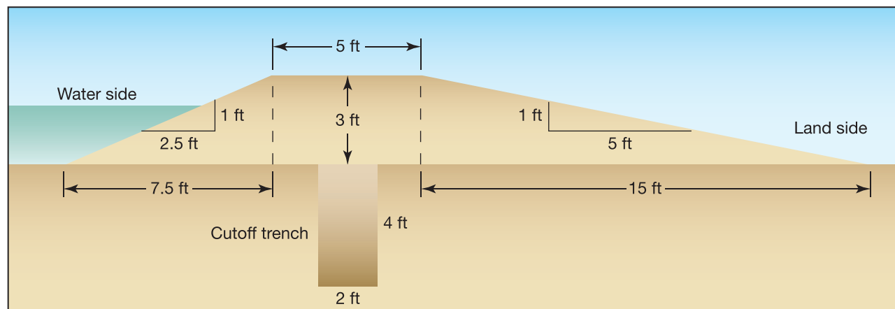
Figure 6-48. Valley House levee cross-sectional dimensions
