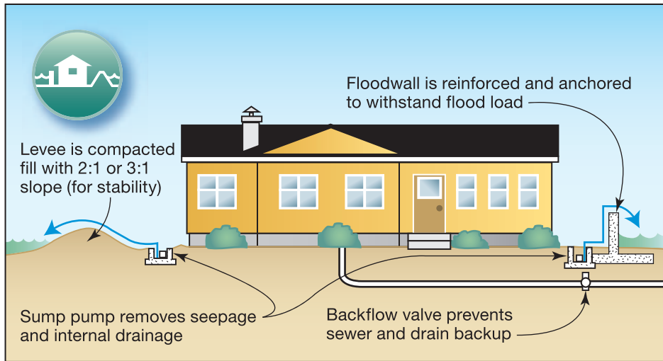
Figure 1-11. Structure protected by floodwall and levee
