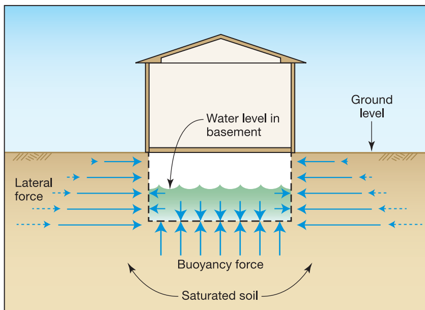
Figure 3-9. Lateral and buoyancy forces resulting from saturated soil
