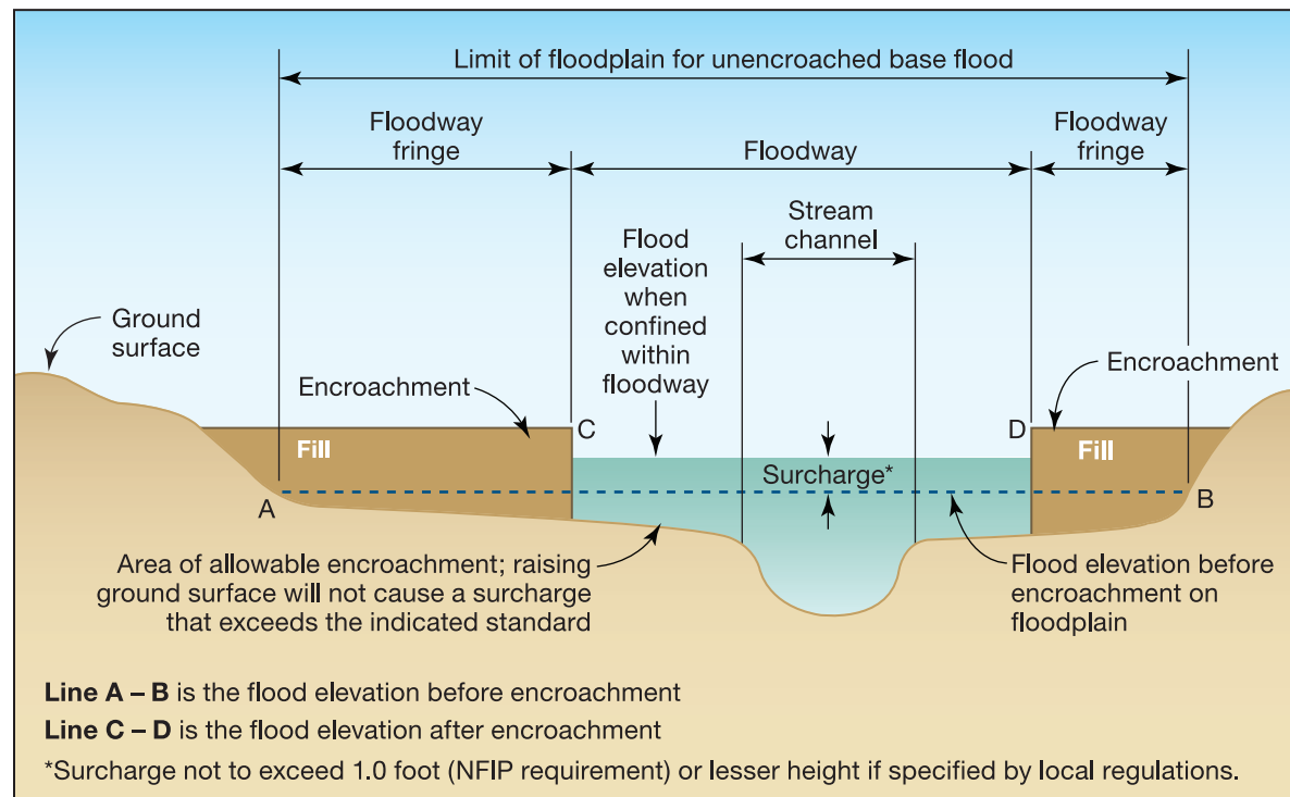
Figure 2-3. Typical riverine floodplain cross section
