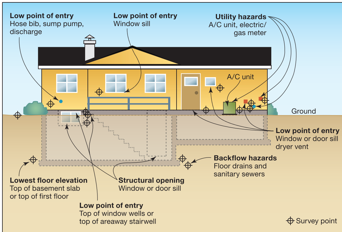
Figure 3-2. Survey to identify the low point of floodwater entry into a typical residential structure
